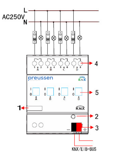
▲ Figure 3: Connection diagram SwitchME4 KNX
