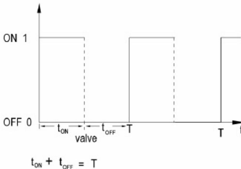
▲ Figure 29: PWM control application
