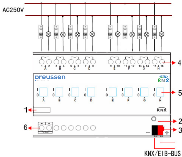
▲ Figure 4: Connection diagram SwitchME8 KNX
